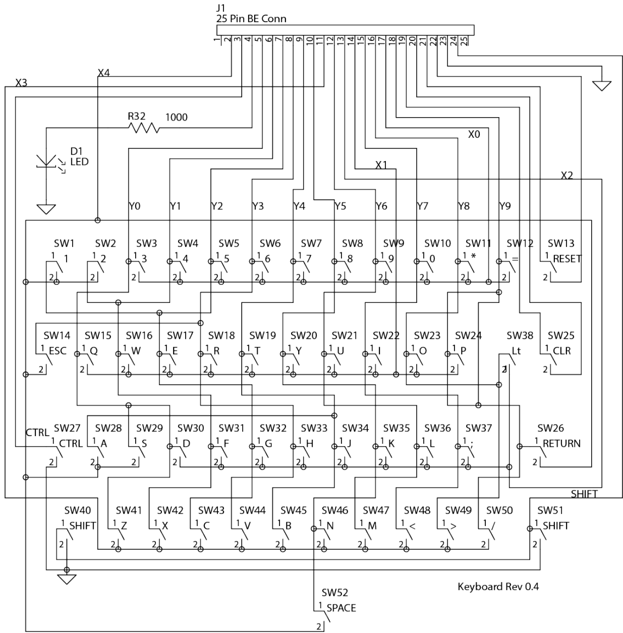
Keyboard 0 Schematic
