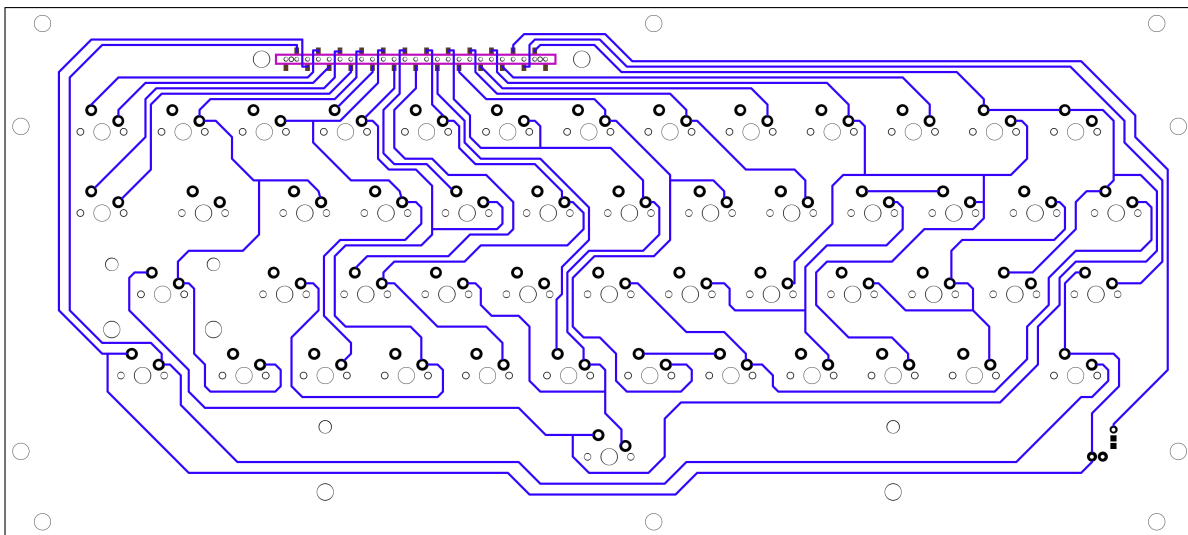
Keyboard 0 Top Assembly
