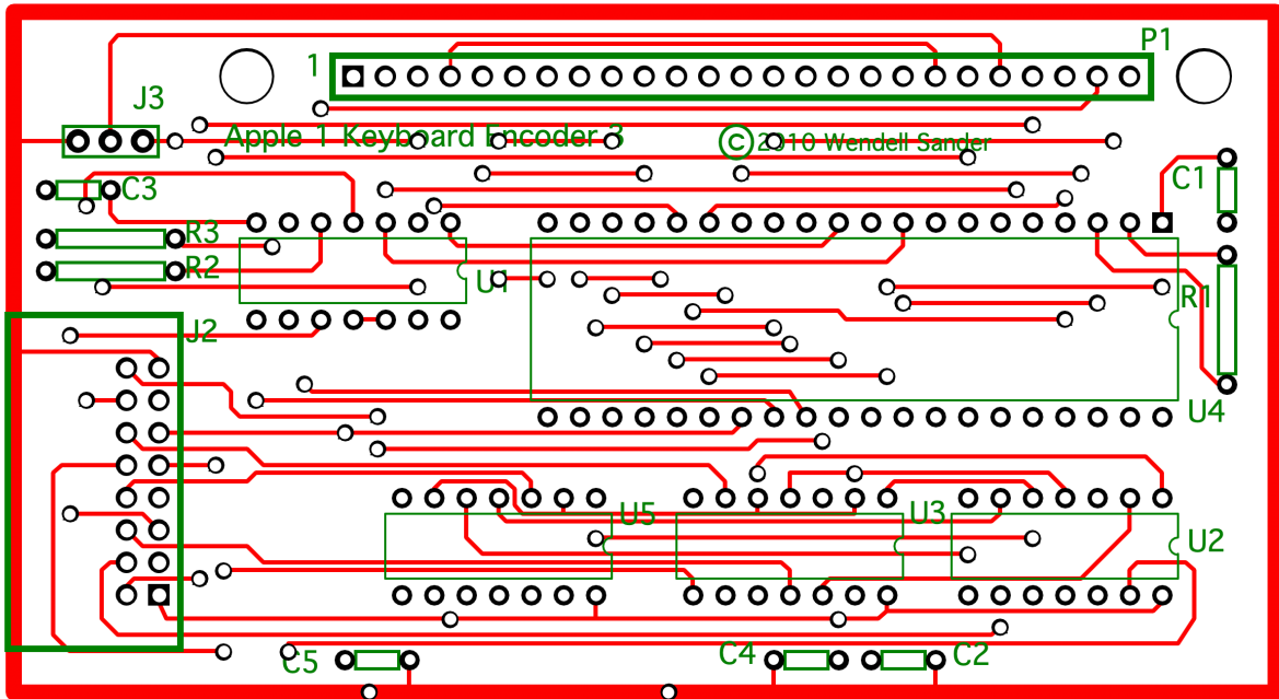
A1 Interface Board Top Assembly
