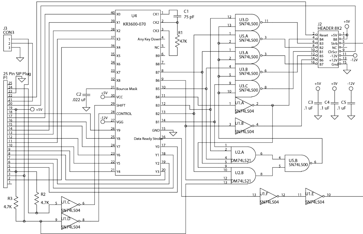
A1 Interface Board Schematic
