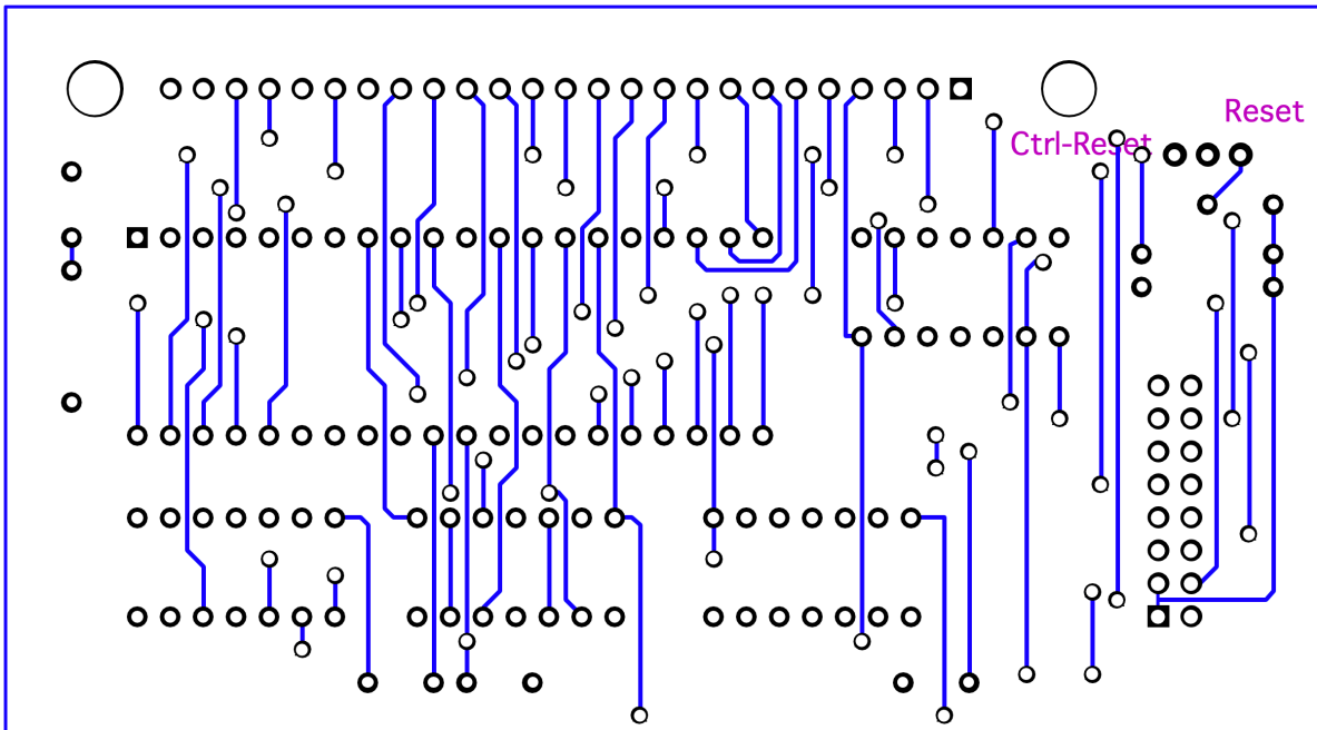
A1 Interface Board Bottom Assembly
